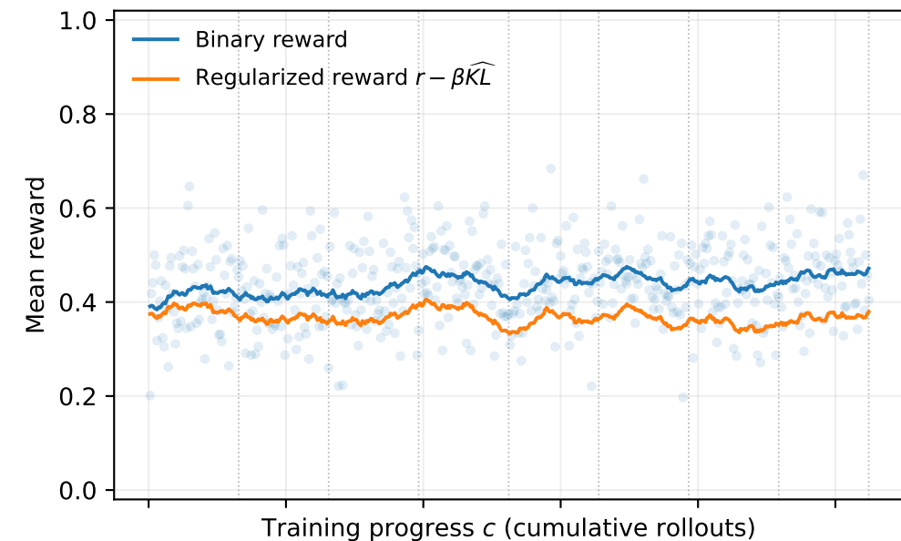
RLOO pilot diagnostics: \beta = 0.2 , G = 32 (32-step rolling means; dots are training batches)
