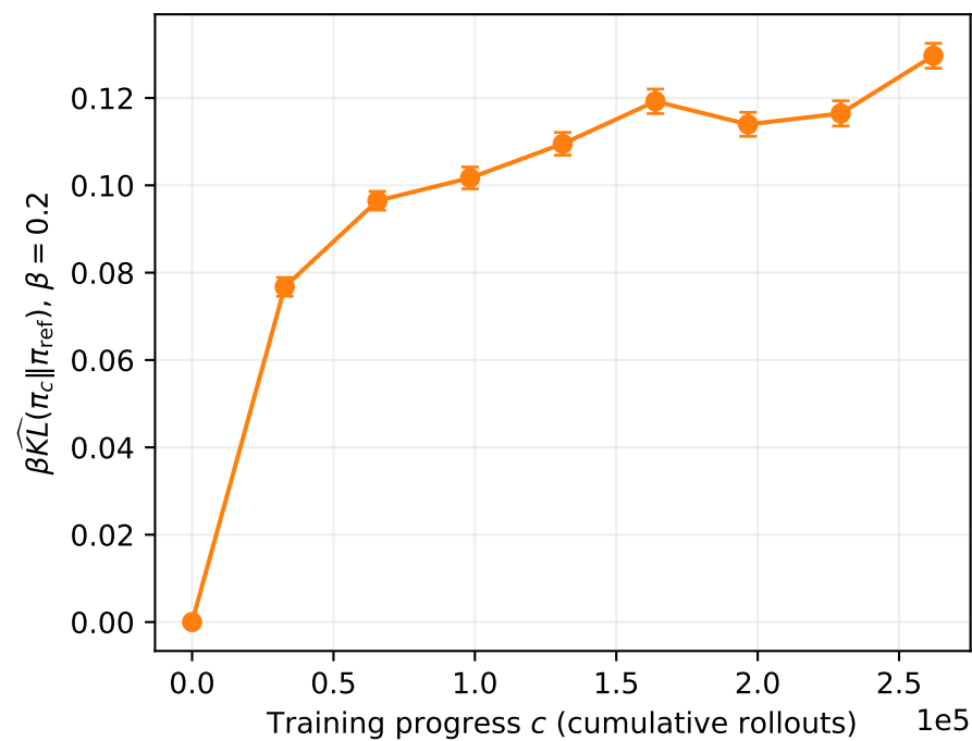
Free-energy decomposition: RLOO, \beta = 0.2 (held-out validation, paired checkpoints)
