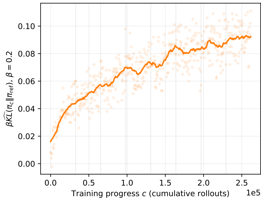
Free-energy decomposition: RLOO, \beta = 0.2 (on-policy training batches, 32-step rolling mean)
