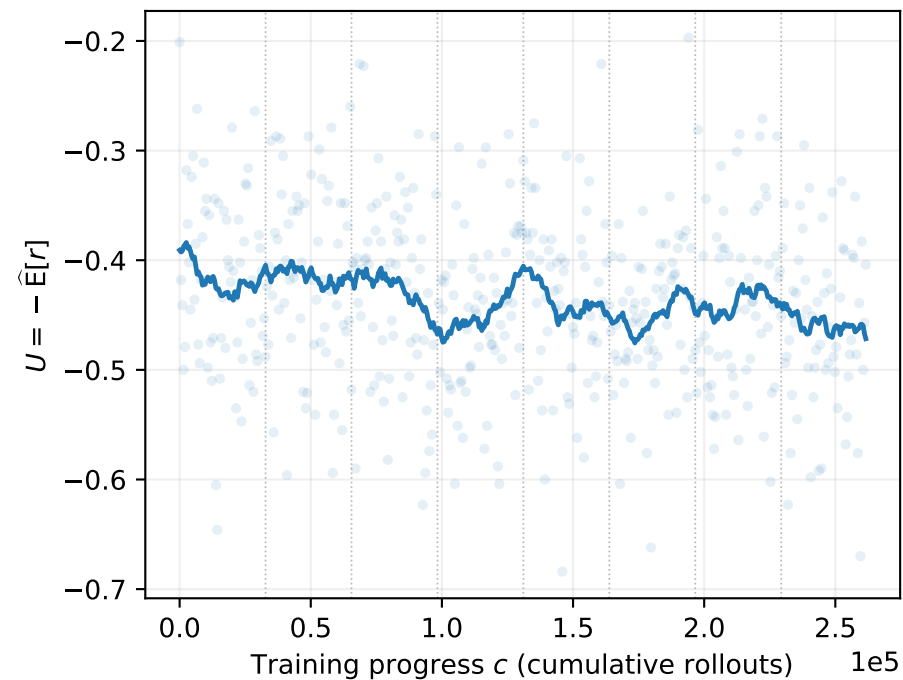
Free-energy decomposition: RLOO, \beta = 0.2 (on-policy training batches, 32-step rolling mean)
