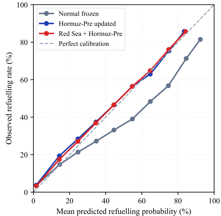
(a) Reliability diagram (deciles)
