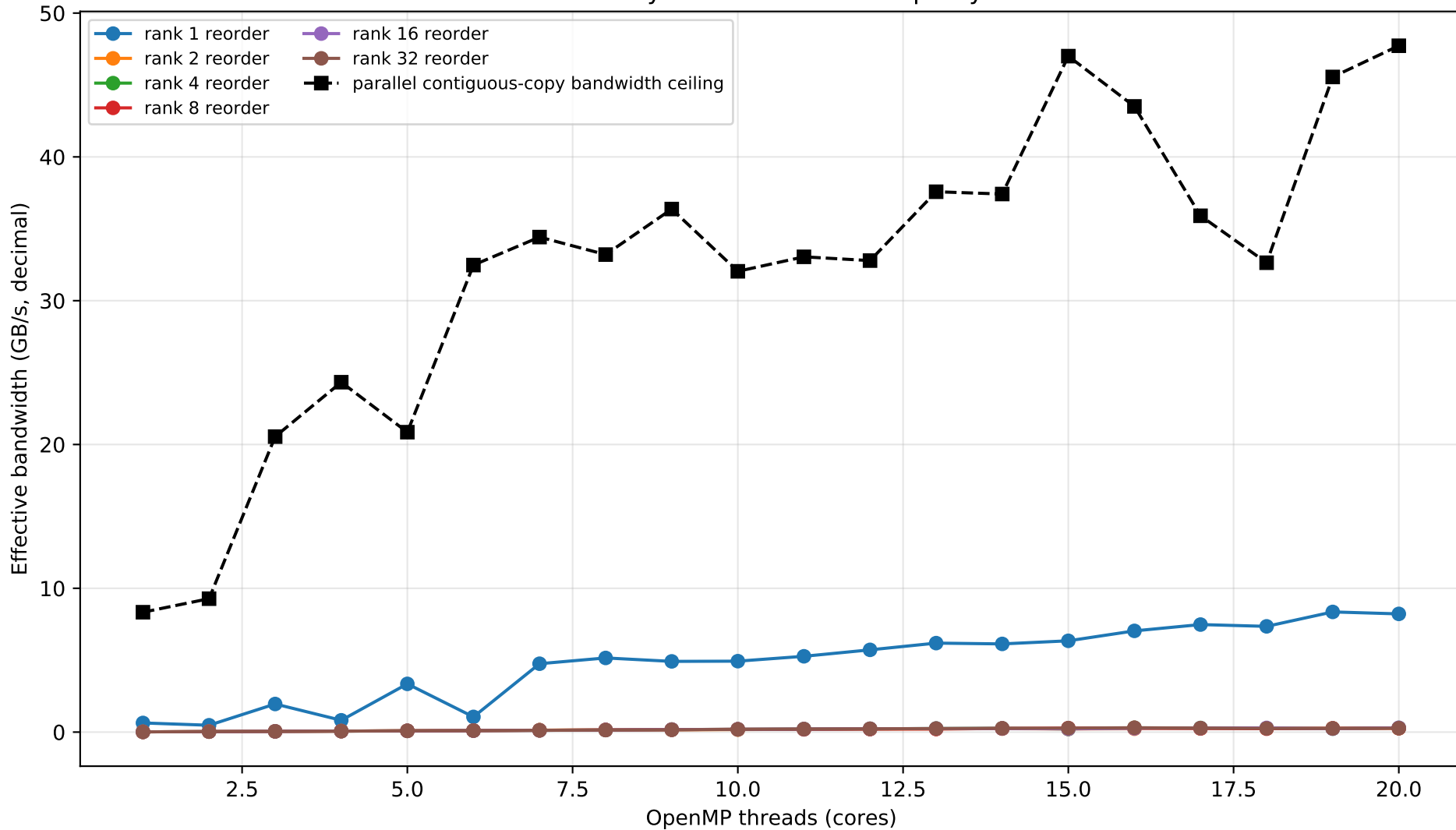
Memory-bandwidth roofline proxy
