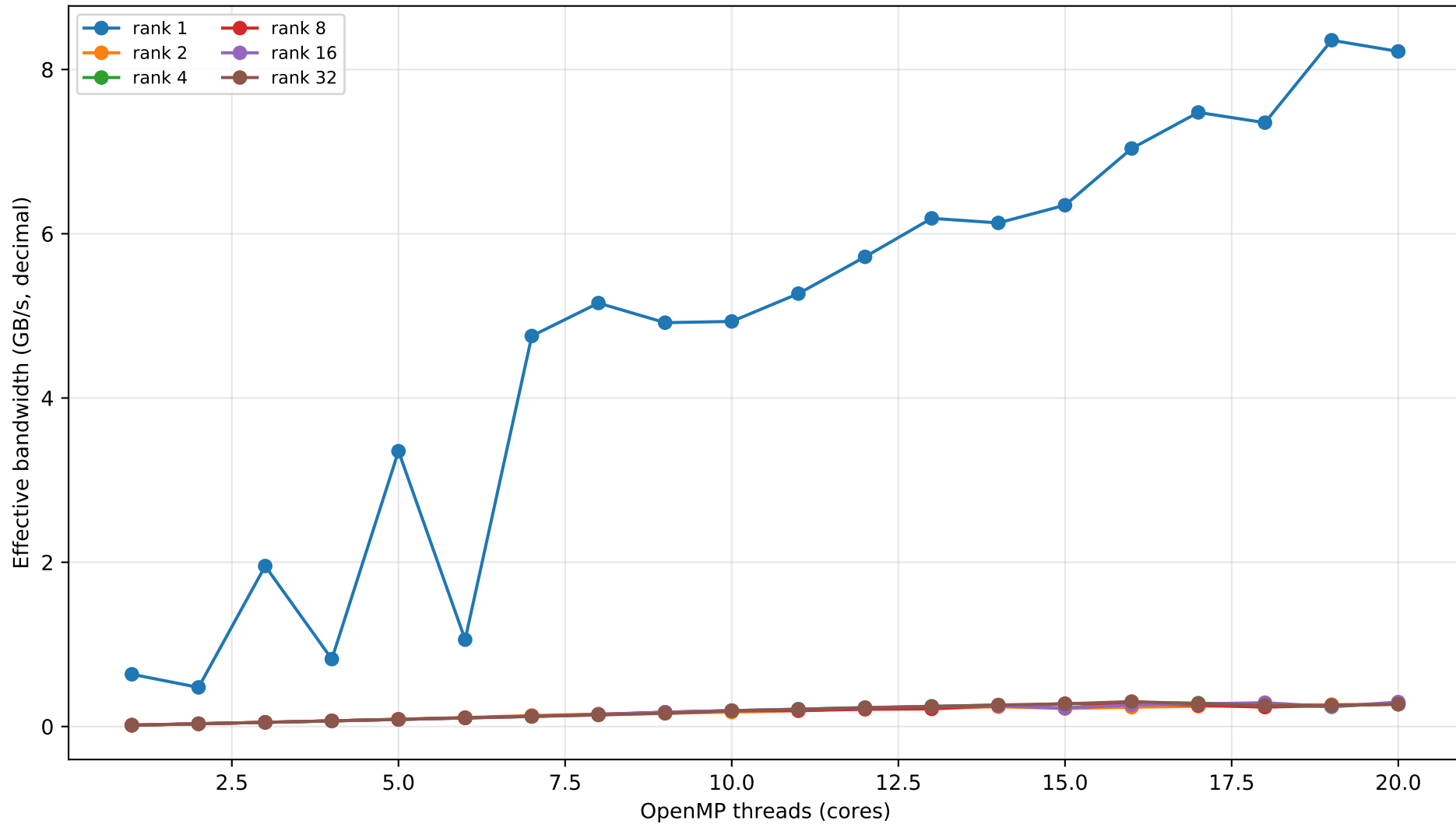
Tensor reorder bandwidth by rank and core count
