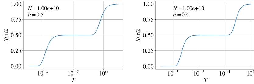
Figure 3: The trend of thermal entropy per spin with temperature, calculated by definition S = \ln Z - \beta \frac{\partial}{\partial \beta} \ln Z directly. The system is the Kitaev model in the toric code limit. The size of the system is fixed to be N = 10^{10} . The melting point of the free-spinon phase does not depend on the value of \alpha . On the other hand, the melting point of the static-flux phase changes significantly when we vary \alpha .
