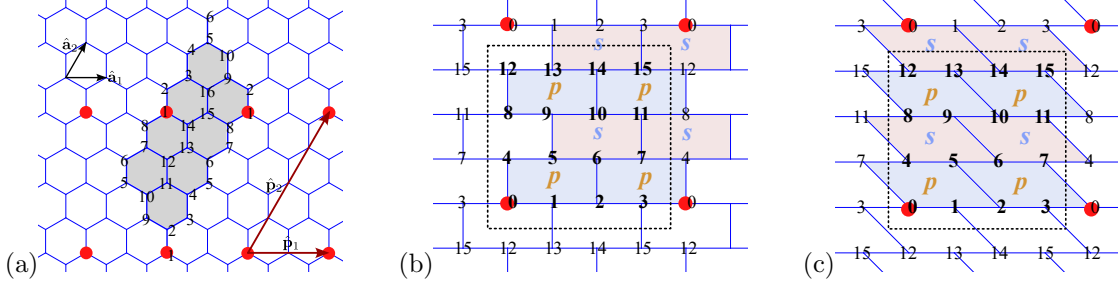
Figure 1: (a) The smallest topologically non-trivial system consists of 8 unit cells, which is equivalent to 16 spins. The two vectors that define the periodic boundary condition are \hat{p}_1 = 2\hat{a}_1 and \hat{p}_2 = 4\hat{a}_2 , respectively. (b) For numerical simplicity, the honeycomb lattice is rearranged into a brick-wall geometry, and the spins are relabeled according to their Euclidean coordinates in the lattice. In both figures, red dots indicate identical lattice sites. (c) An equivalent choice.
