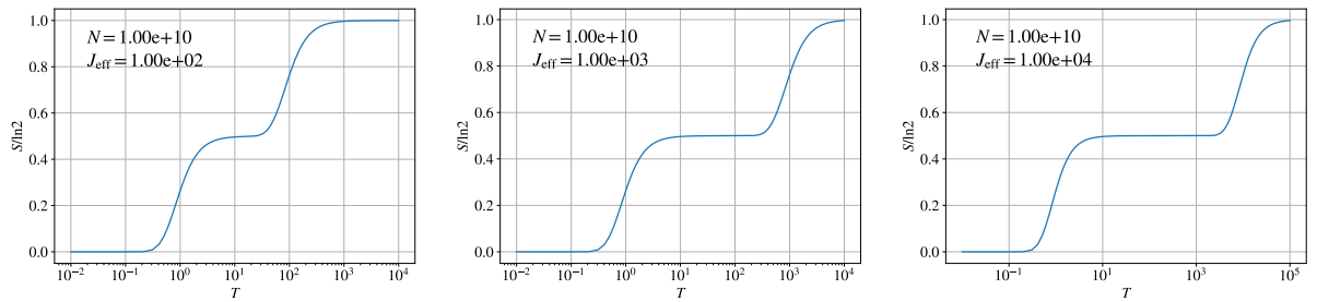
Figure 3: The trend of thermal entropy per spin with temperature, calculated by definition S = \ln Z - \beta \frac{\partial}{\partial \beta} \ln Z directly. The system is the Kitaev model in the toric code limit. The size of the system is fixed to be N = 10^{10} , and J_{\text{eff}} is the coupling constant of the low-energy effective theory appearing in Eq. (8.8). The melting point of the static-flux phase does not depend on the value of J_{\text{eff}} . On the other hand, the melting point of the free-spinon phase changes significantly when we vary J_{\text{eff}} .
