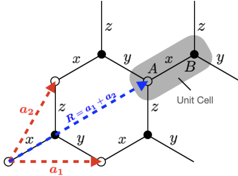
FIG. 10. A 2 \times 2 honeycomb lattice with sublattices A and B . The A sites form a triangular lattice with primitive vectors \mathbf{a}_1 and \mathbf{a}_2 . Each unit cell (denoted by \mathbf{R} ) contains one spin from both sublattices joined by an x -link. A reference unit cell is illustrated in the figure.
