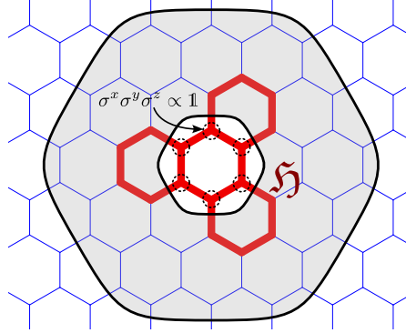
Figure 1: The patch configuration \mathfrak{H} covering the interior hole of a non-simply connected subsystem. This configuration is devised in such a way that the corresponding string operator \Sigma_{\mathfrak{H}} has all its local components inside the hole B equal to the identity. Its corresponding string operator \Sigma_{\mathfrak{H}} commutes with other string operators lying within the shaded subsystem.
