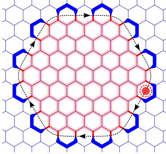
Figure 4: In the Kitaev model, assembling \xi -operators along a closed loop represents a 't Hooft loop of the \mathbb{Z}_2 gauge theory, which can be understood as the path of a \mathbb{Z}_2 gauge flux (vison) moving along the closed loop and eventually being annihilated by its partner created at the same spot at the very beginning. It is also equivalent to the subsystem fermion parity of the region enclosed by the 't Hooft loop.
