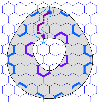
Figure 2: An unsolved problem is the pattern of patch sectors of subsystems with both their inner and outer boundaries having odd length. In this case, there is no well-defined \Xi operator, but the \xi operators surrounding the inner boundary cannot form a valid patch configuration either. A possible resolution is to connect the remaining sites at the inner and outer boundaries. One example is the Wilson operator enclosed by the dashed frame in the above illustration. However, this method also requires the \xi operators along the outer boundary, which should not be included in this framework.
