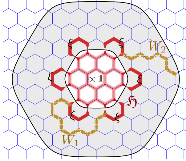
Figure 3: The non-contractible Wilson operator W_2 with two endpoints attached to different boundaries anti-commutes with the patch operator \Sigma_{\mathfrak{H}} covering the interior hole, which is proportional to the product of all the \xi operators surrounding the inner boundary, while the non-contractible Wilson operator W_1 with both endpoints attached to the patch commutes with \Sigma_{\mathfrak{H}} as well as other string operators supported within the subsystem A , hence commutes with the reduced density matrix \rho_A .
