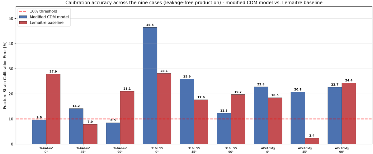
Figure 5: Fracture strain calibration errors of the modified CDM model (blue) and the conventional Lemaitre baseline (red) for each of the nine calibration cases, both under the leakage-free parameterization: single S_0 per material, literature g_s , no orientation multipliers; the baseline shares the identical 20-grain Taylor aggregate, hardening and texture ( f_{AM} \equiv 1 ). The dashed line indicates the 10% accuracy target. In calibration the baseline averages 18.6% over the nine cases versus 20.4% for the modified model; in the strict blind cross-validation (Table 5) the averages are 24.3% (baseline) versus 31.2% (modified), and the information criteria favor the baseline at equal parameter count as an auxiliary descriptive margin (Section 5), but a paired test of the nine blind folds cannot distinguish the two models—the modified model adds directional information rather than a reduction of the mean error.
