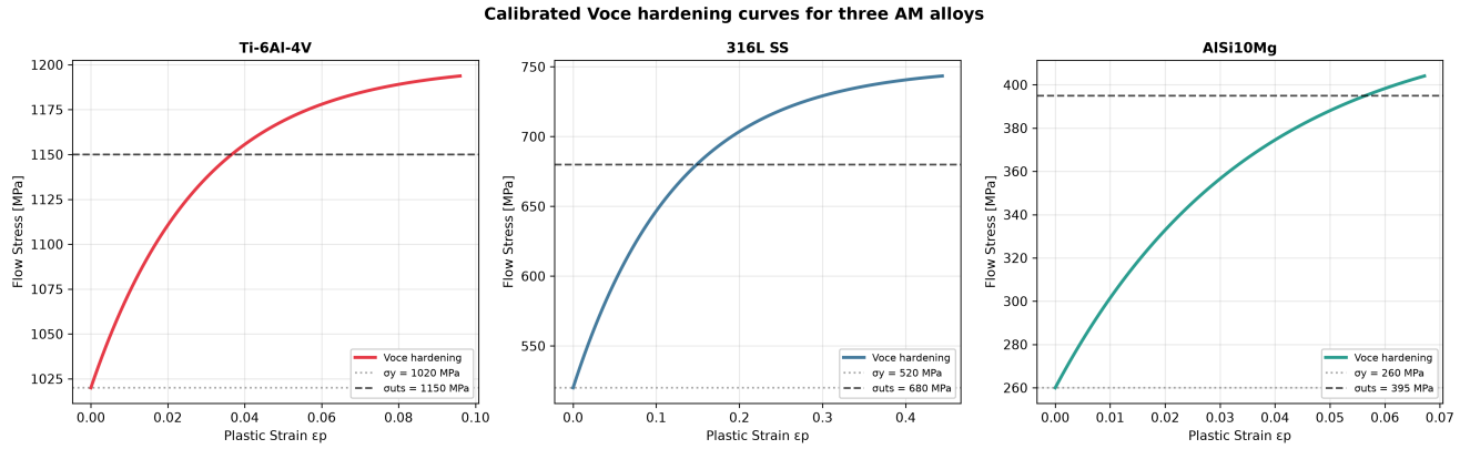
Figure 2. Voce hardening curves of the three AM alloys with the literature-fixed parameters of Table 1. The curves are not fitted to fracture data; the flow response follows from the fixed hardening constants.
