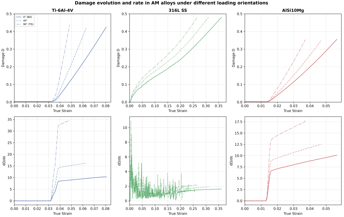
Figure 1. Orientation-dependent damage response that the AM descriptors are designed to capture: predicted damage D (top row) and damage rate dD/d\varepsilon (bottom row) versus true strain for the three AM alloys (Ti-6Al-4V, 316L SS, AISi10Mg) at loading angles 0^\circ (build direction), 45^\circ and 90^\circ (transverse direction). For every alloy the transverse 90^\circ orientation accumulates damage fastest, reaching a given damage level at the smallest strain—the orientation-dependent acceleration that the descriptors introduced below are constructed to represent.
