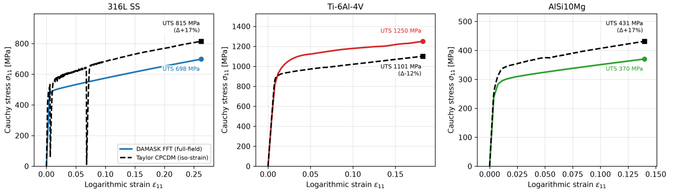
Figure 8. Damage-free macroscopic response of the Taylor iso-strain model (dashed) versus the DAMASK spectral-FFT full-field reference (solid) for the three alloys under identical 30-grain microstructures. Markers indicate the respective UTS.
