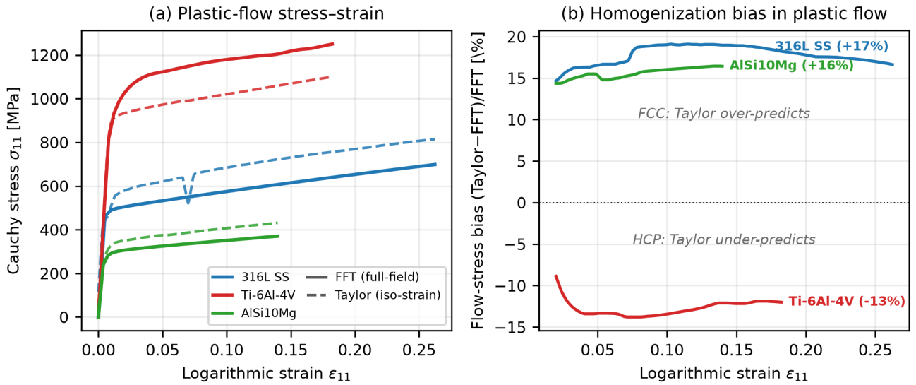
Figure 9. Taylor iso-strain (dashed) versus DAMASK spectral-FFT full-field (solid) plastic-flow response, damage-free, loading along the build direction. (a) True (Cauchy) stress against logarithmic strain for the three alloys; the surrogate misrepresents the flow-stress level throughout the plastic branch, not only at the UTS. (b) Resulting flow-stress bias (\sigma^{\text{Taylor}} - \sigma^{\text{FFT}})/\sigma^{\text{FFT}} as a function of plastic strain: the FCC alloys are over-predicted (+15 to +19%) and the HCP Ti-6Al-4V under-predicted (−11 to −14%), and the monotone drift of each curve with strain is the hardening-rate bias (Table 7).
