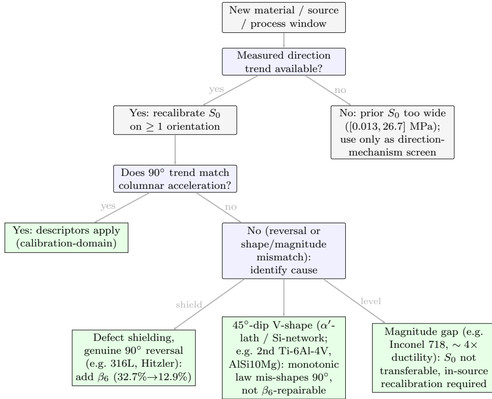
Figure 7. Decision procedure for applying the damage descriptors to a material, source or process window not in the calibration set. The branches are keyed to the failure-mode classification of Table 6; the 45°-residual case (second AlSi10Mg) is a boundary of the projection laws inside the mechanism class and is covered by the mechanism-consistency check of step 2.
