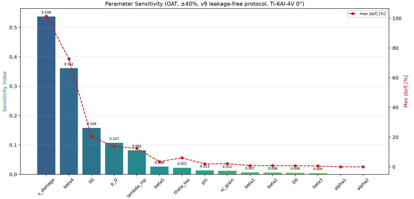
Figure 6. One-at-a-time (OAT) sensitivity of the predicted fracture strain to \pm 40\% variations of each damage-model parameter (Ti-6Al-4V, 0^\circ , production leakage-free parameters).
