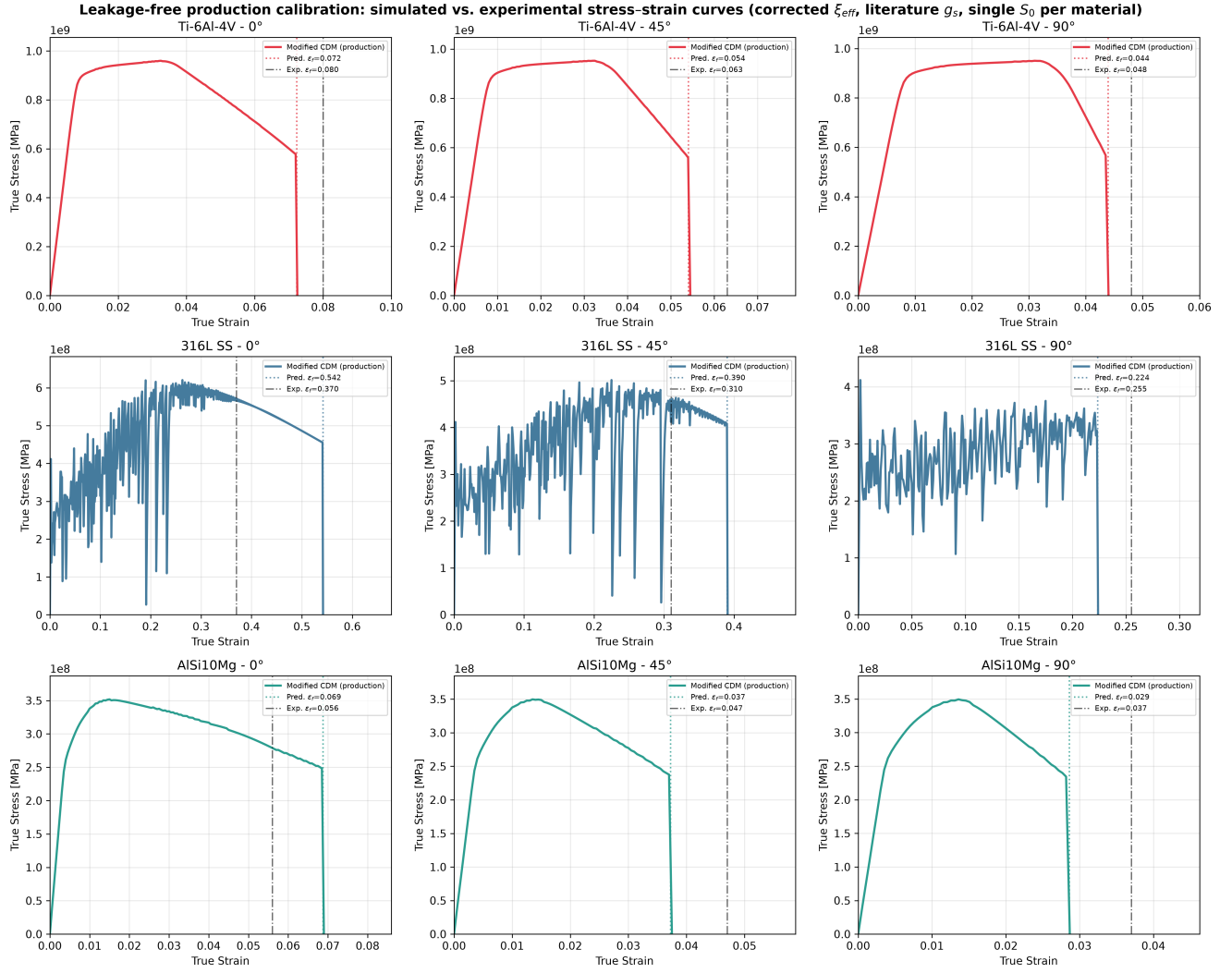
Figure 3. True stress–strain curves predicted by the modified CDM model for all nine calibration cases (three materials \times three build orientations). The vertical dash–dotted and dotted lines mark the experimental and predicted fracture strains, respectively, in each panel.
