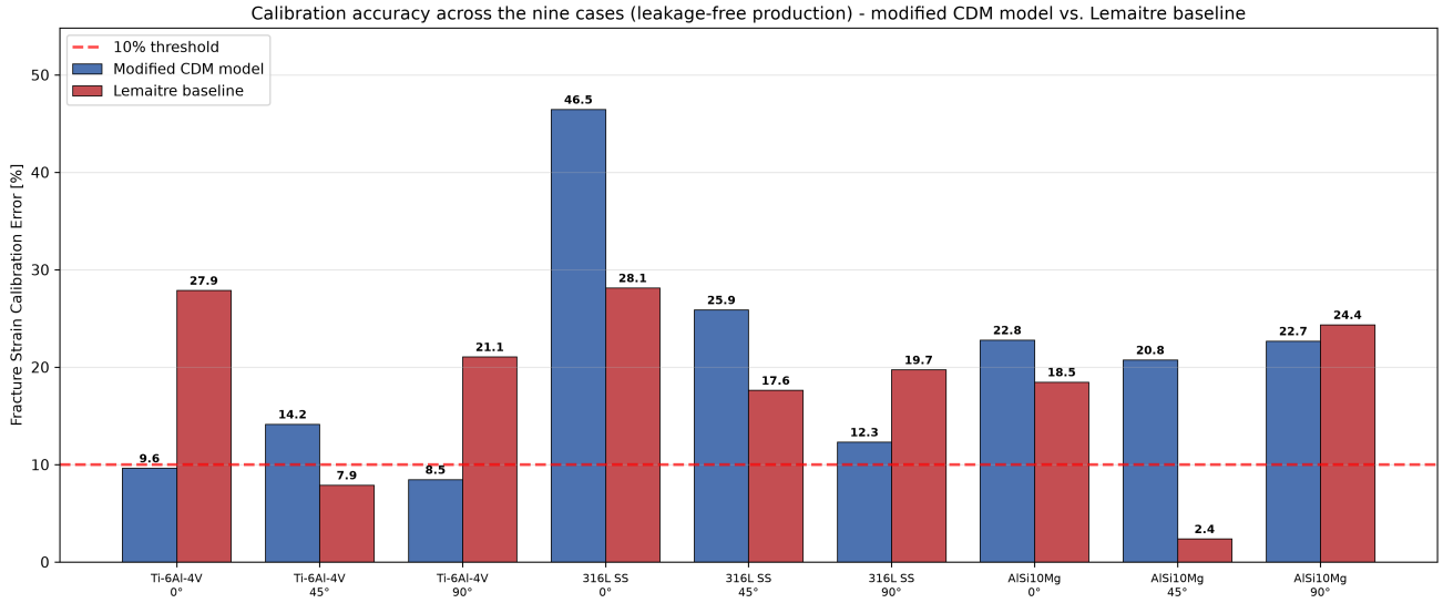
Figure 5. Fracture strain calibration errors of the modified CDM model (blue) and the conventional Lemaitre baseline (red) for each of the nine calibration cases, both under the leakage-free parameterization: single S_0 per material, literature g_s , no orientation multipliers; the baseline shares the identical 20-grain Taylor aggregate, hardening and texture ( f_{AM} \equiv 1 ). The dashed line indicates the 10% accuracy target. In calibration the baseline averages 18.6% over the nine cases versus 20.4% for the modified model; in the strict blind cross-validation (Table 5) the averages are 24.3% (baseline) versus 31.2% (modified), and the information criteria favor the baseline at equal parameter count as an auxiliary descriptive margin (Section 5), but a paired test of the nine blind folds cannot distinguish the two models—the modified model adds directional information rather than a reduction of the mean error.
