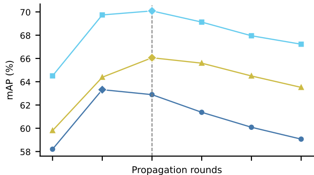
OS-MN40-core
