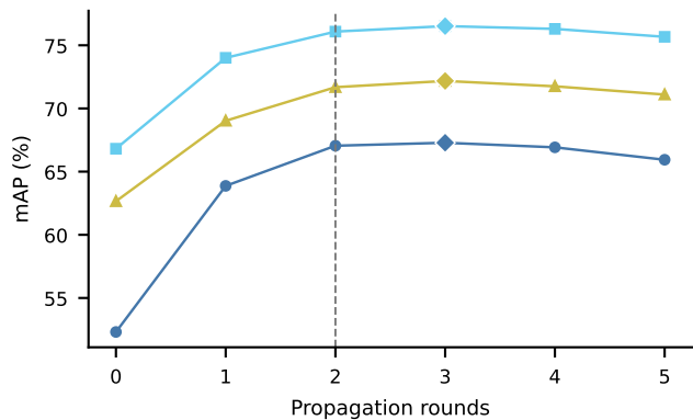
OS-MN40-core
