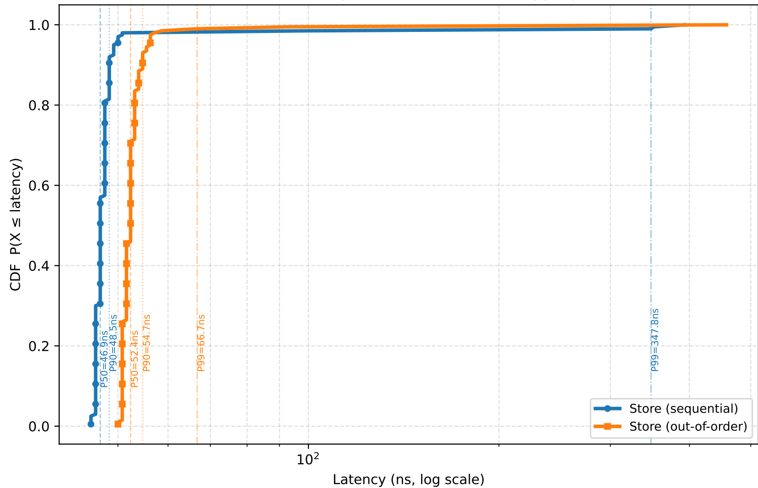
Store Latency CDF — Tiered PSN Mapping
