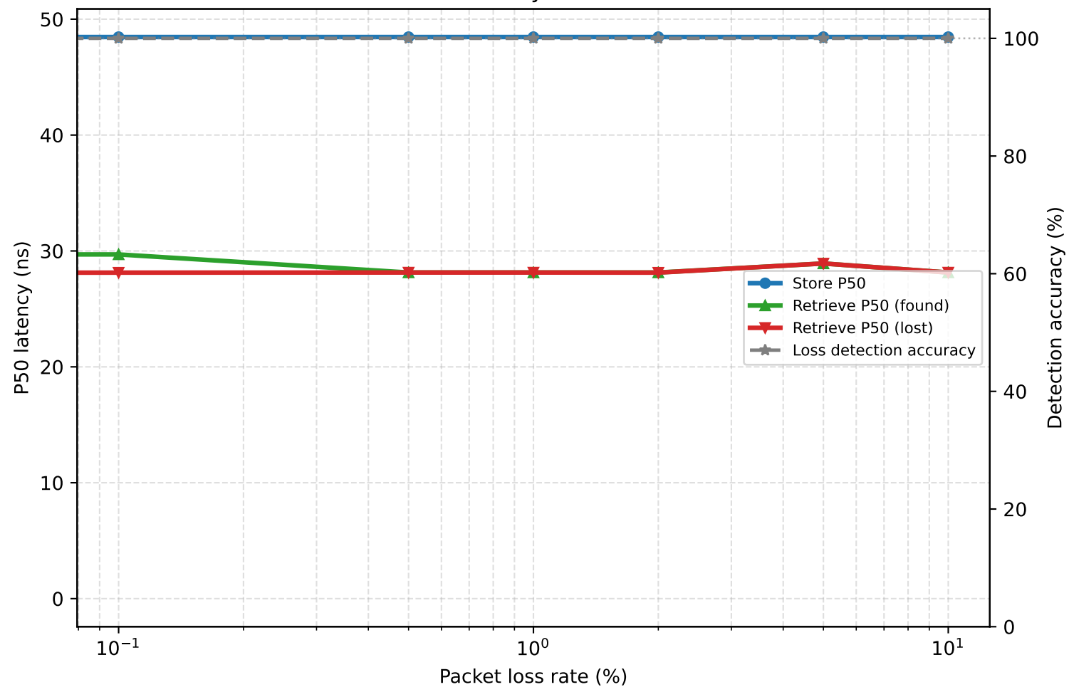
Store/Retrieve Latency vs. Packet Loss Rate
