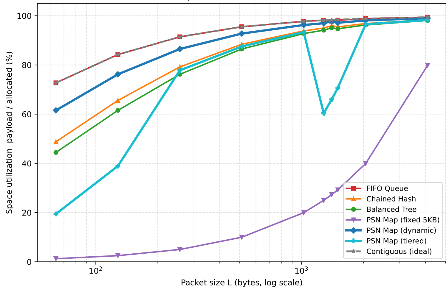
Cache Space Utilization vs. Packet Size
