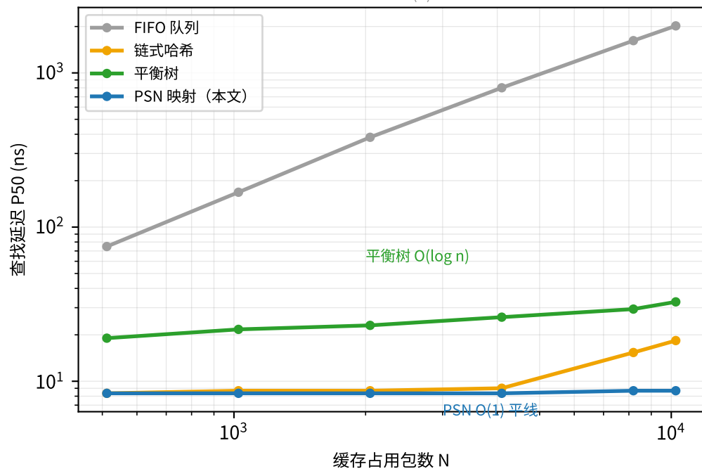
(a) 查找延迟随 N 增长 (复杂度曲线)
