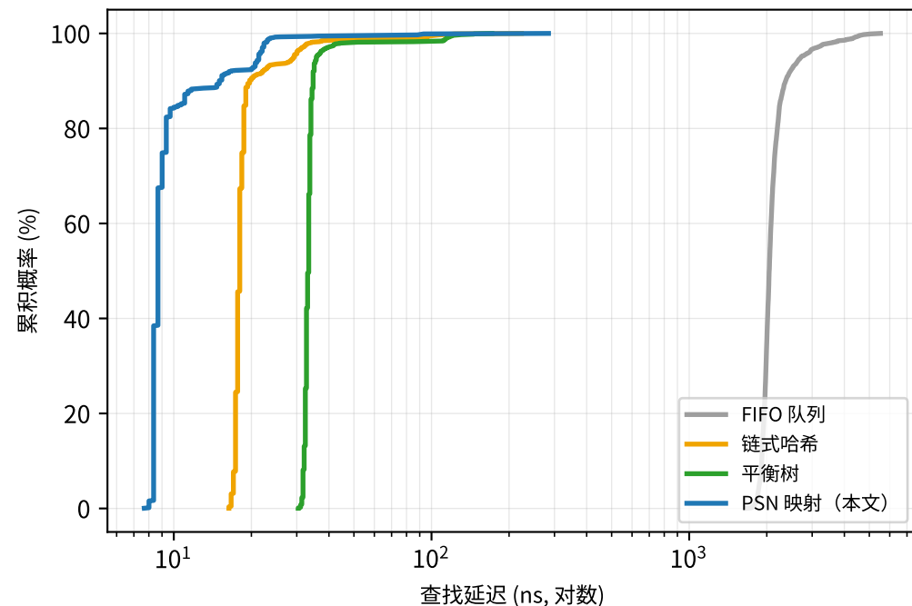
(b) 随机访问查找延迟 CDF
