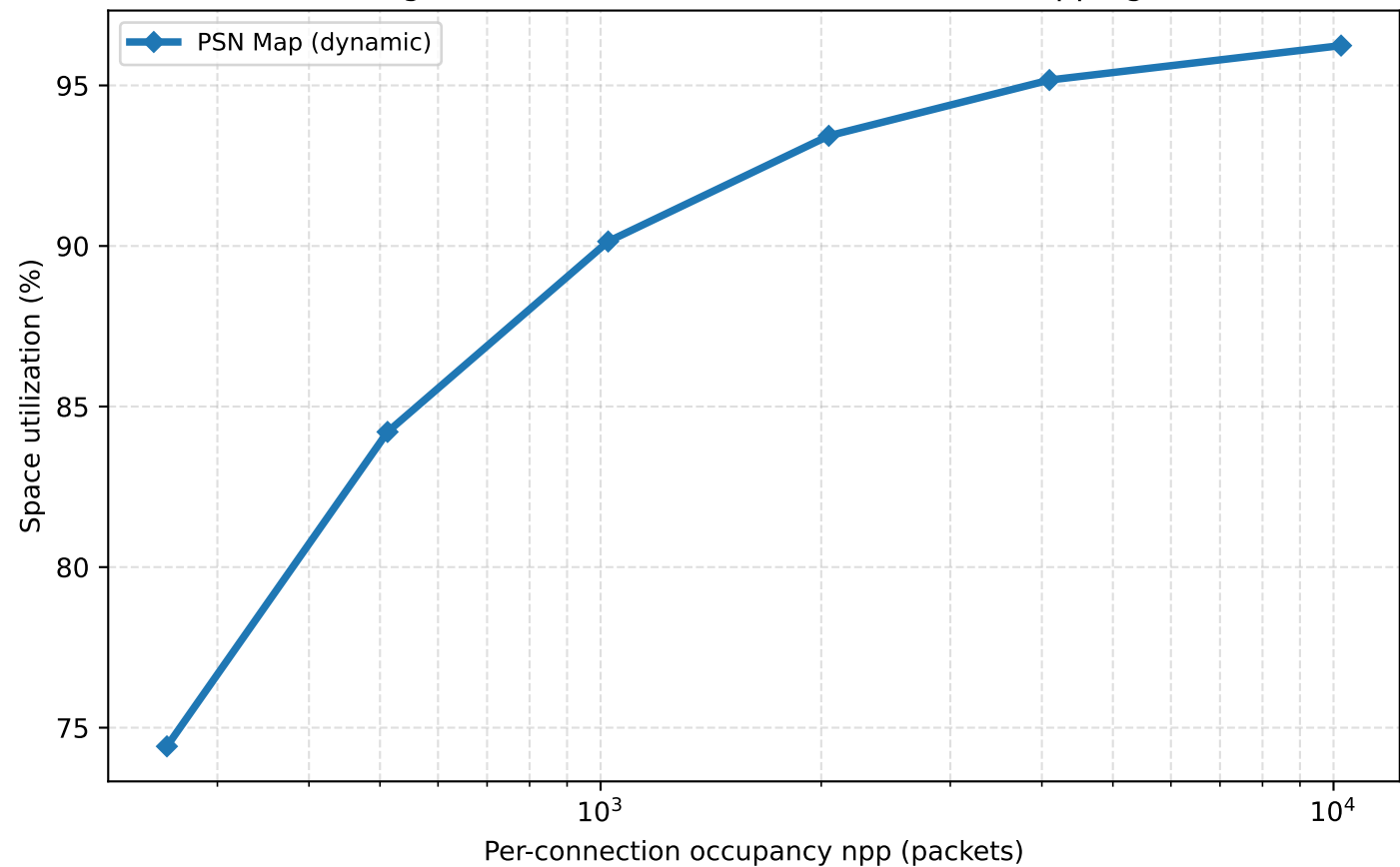
Ring Buffer Overhead Amortization (PSN Mapping)
