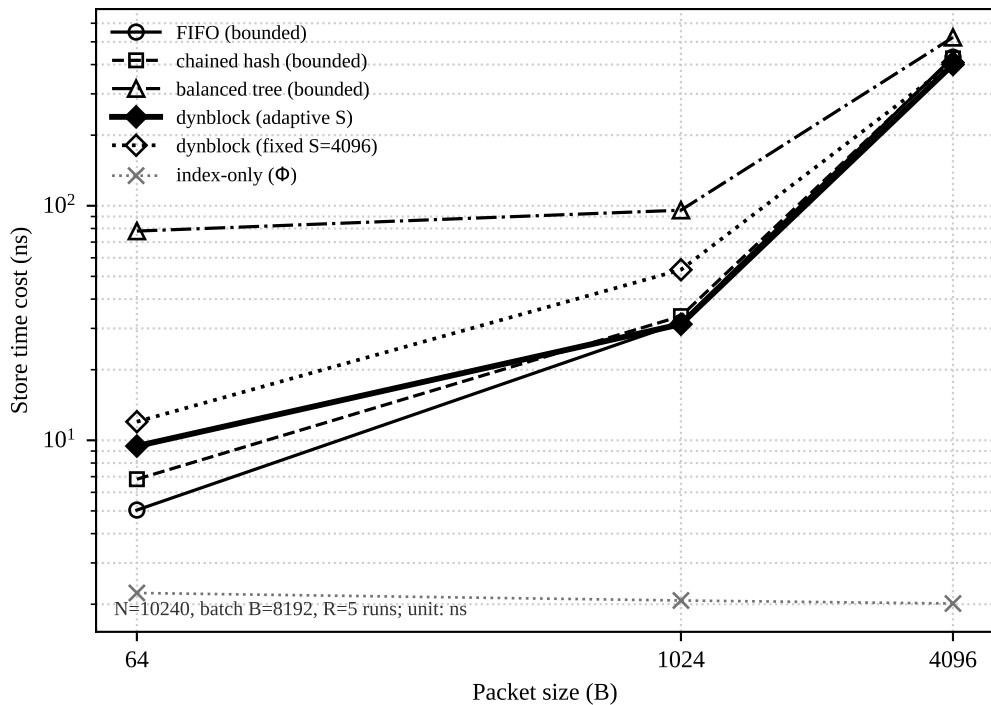
Store time cost versus packet size
