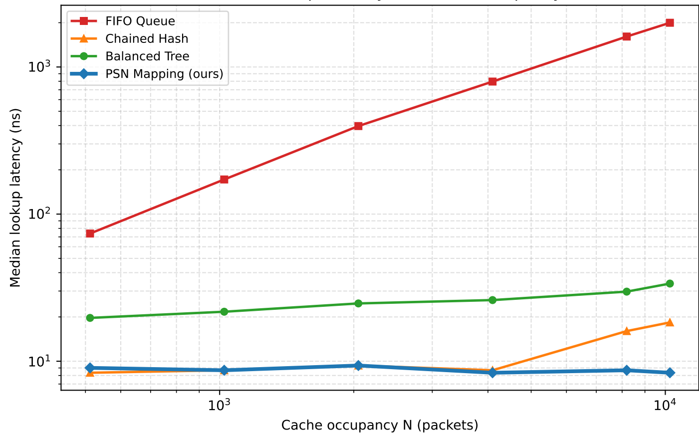
Median Lookup Latency vs. Cache Occupancy
