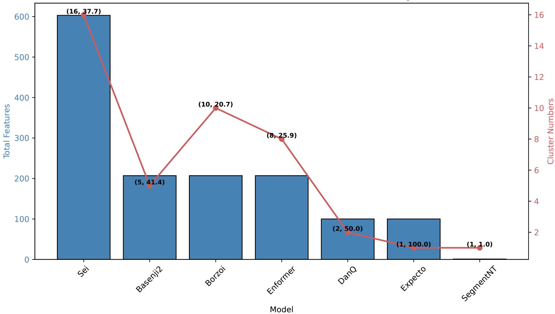
Model Feature Count vs Cluster Numbers and Diversity
