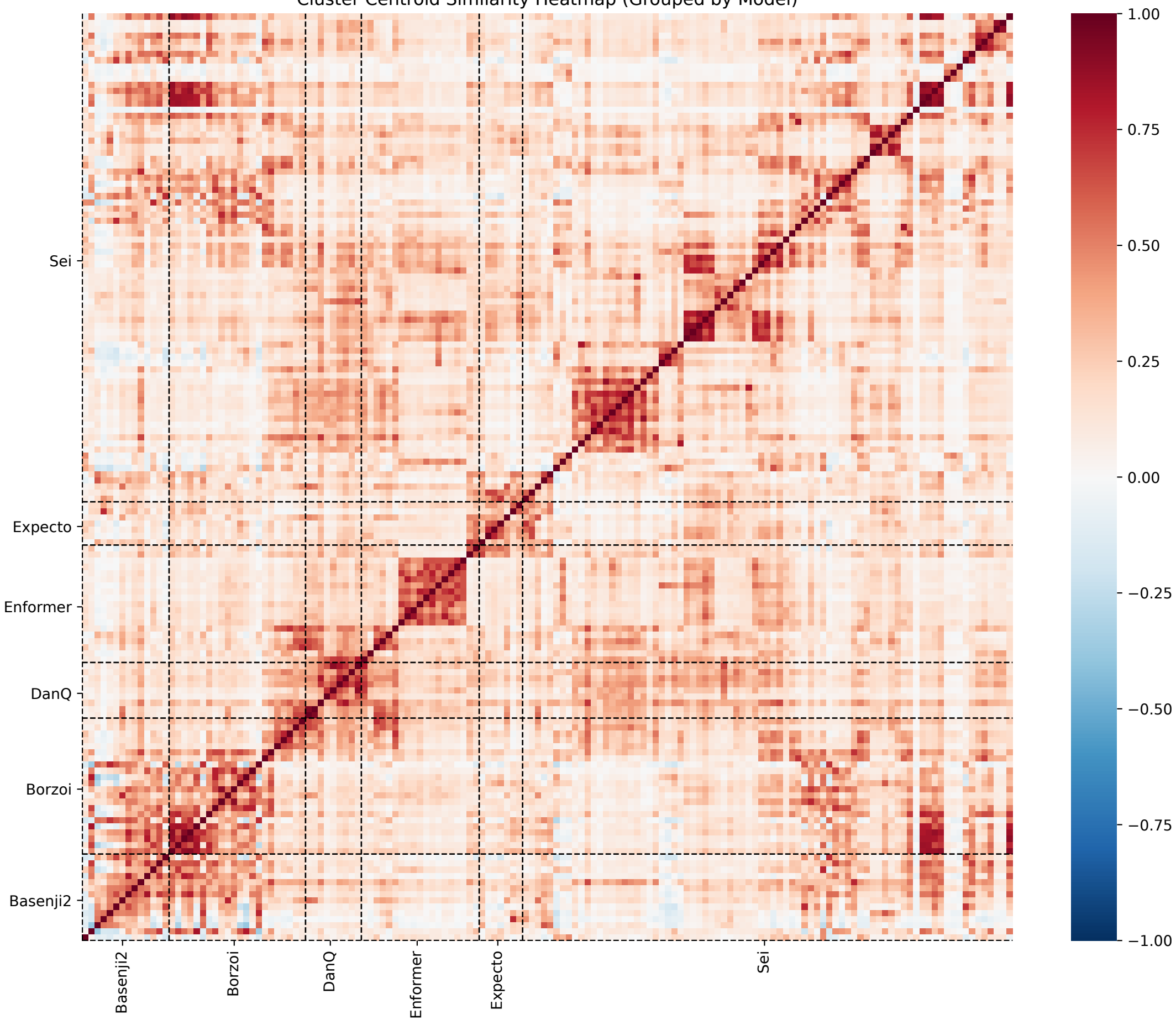
Cluster Centroid Similarity Heatmap (Grouped by Model)
