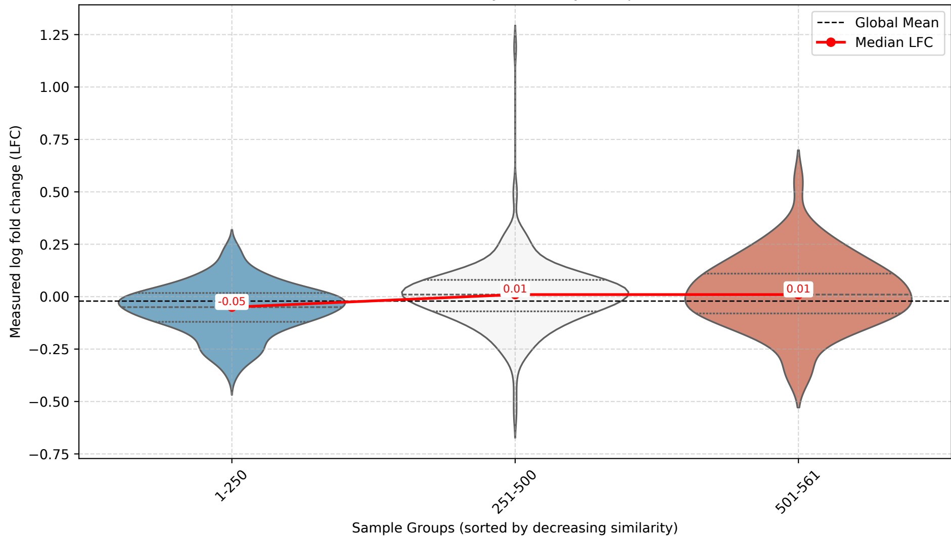
Violin Plot of LFC by Similarity Group (HBB)
