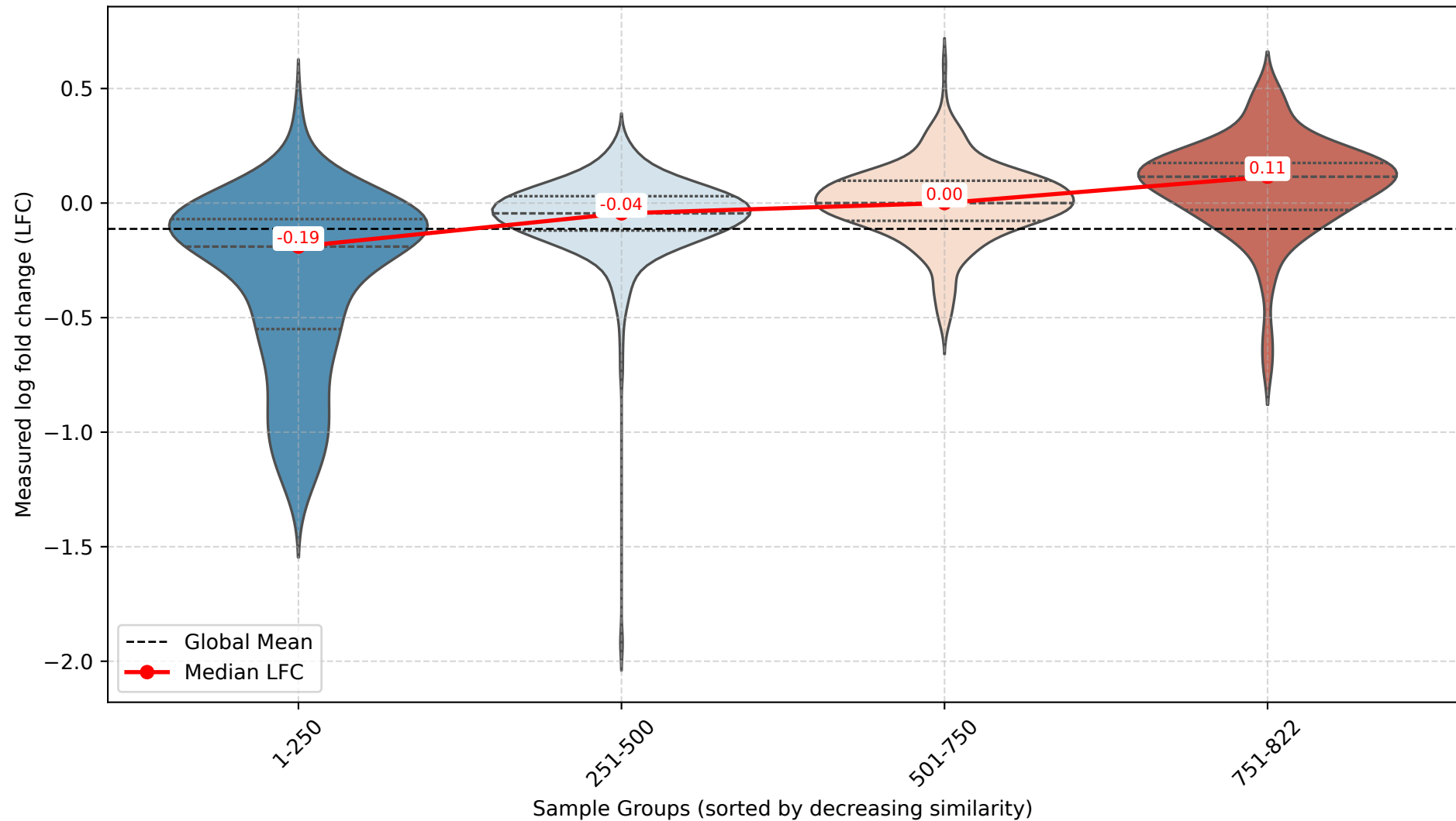
Violin Plot of LFC by Similarity Group (HBG1)
