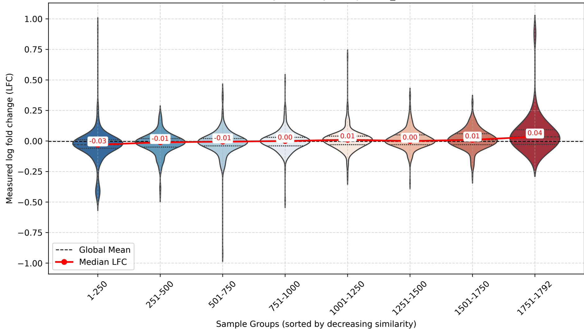
Violin Plot of LFC by Similarity Group (MYC_rs6983267)
