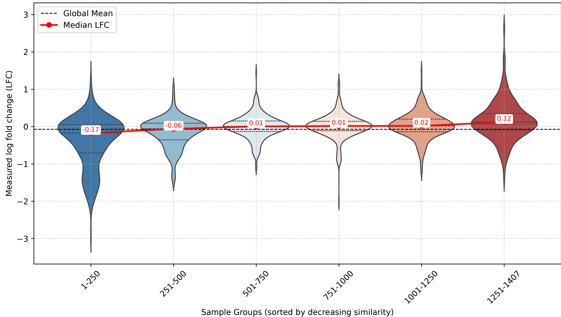
Violin Plot of LFC by Similarity Group (PKLR)
