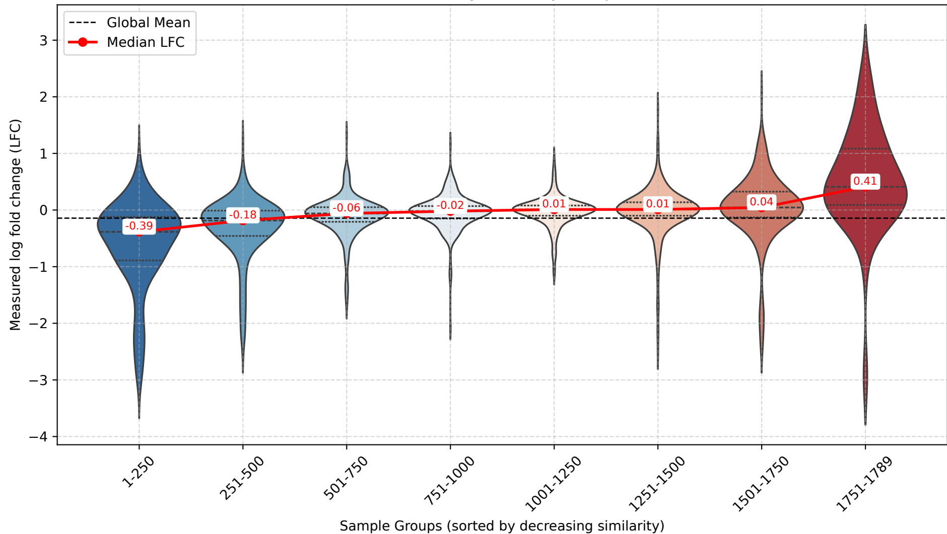
Violin Plot of LFC by Similarity Group (SORT1)
