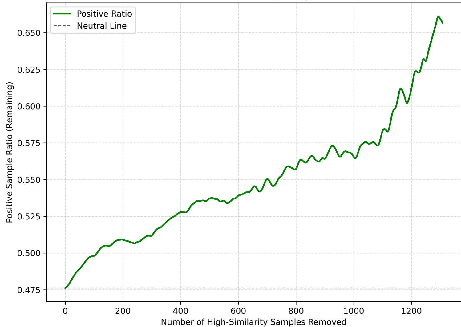
Positive Ratio in Remaining Samples (PKLR)
