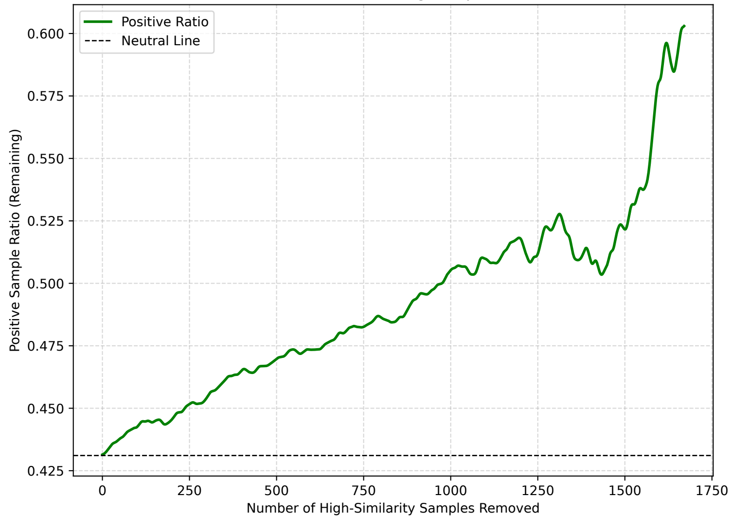
Positive Ratio in Remaining Samples (TCF7L2)
