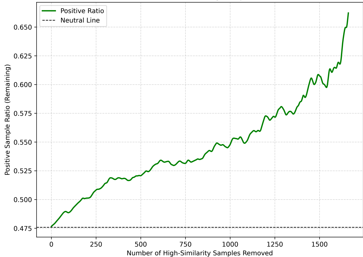
Positive Ratio in Remaining Samples (UC88)
