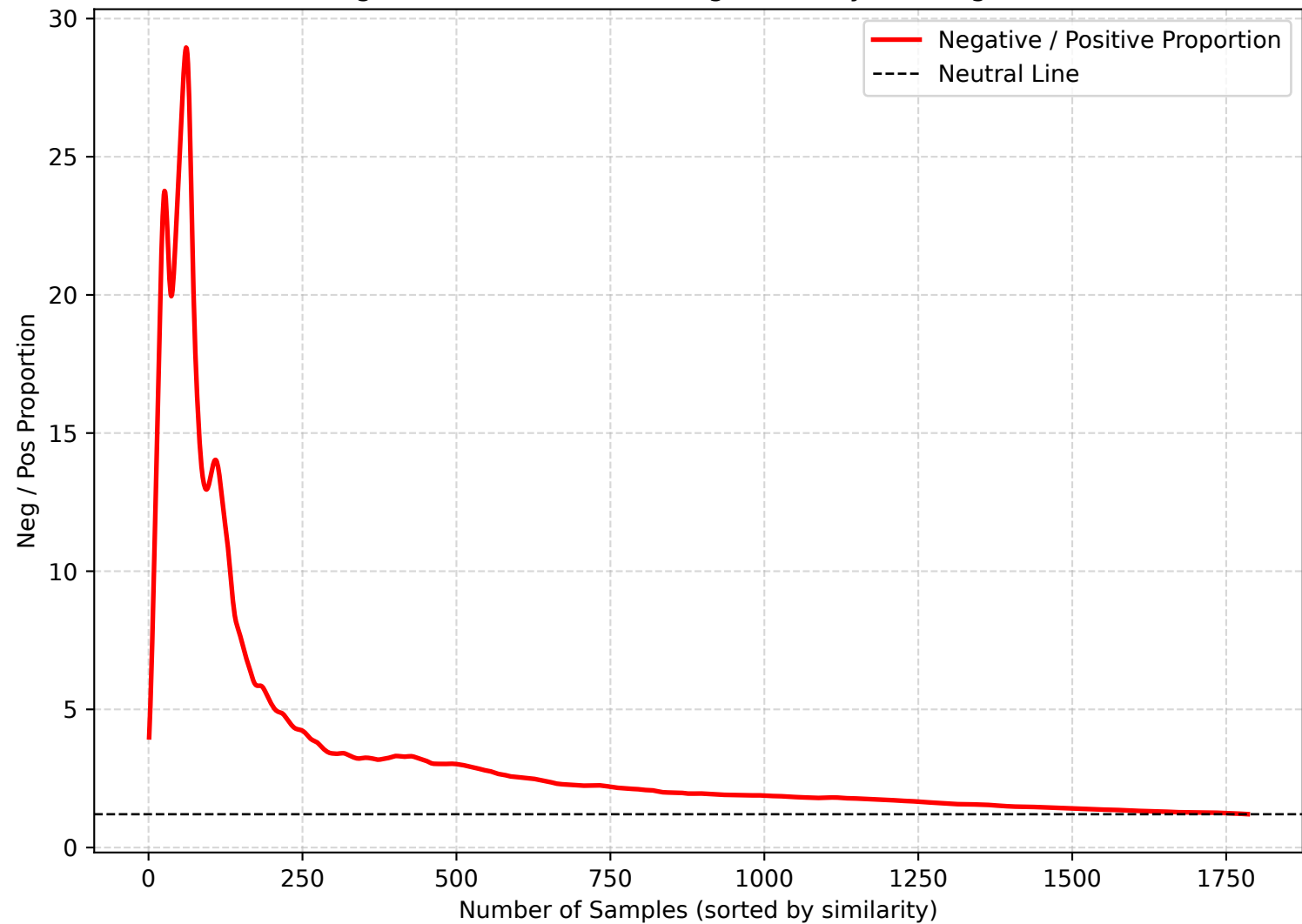
Negative/Positive Ratio along Similarity Ranking (IRF6)
