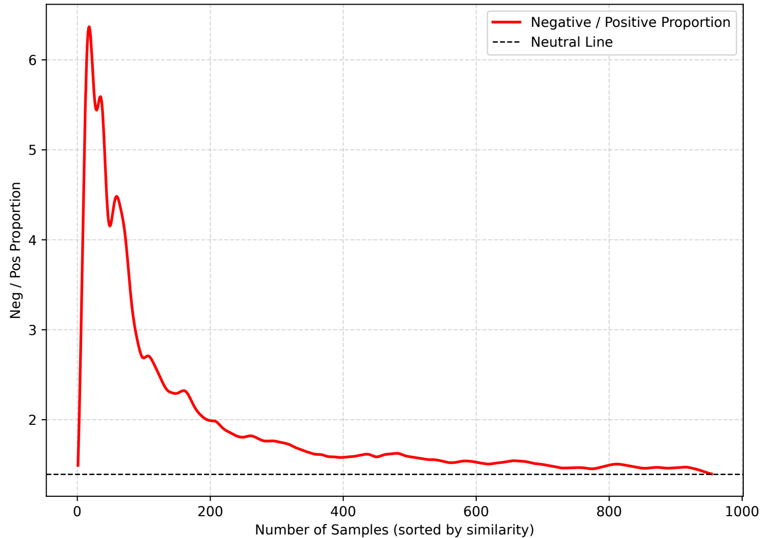
Negative/Positive Ratio along Similarity Ranking (LDLR)
