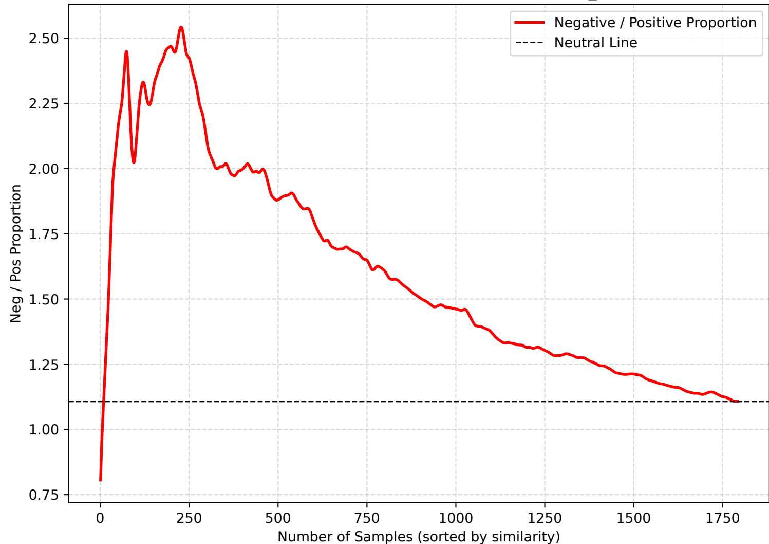
Negative/Positive Ratio along Similarity Ranking (MYC_rs6983267)
