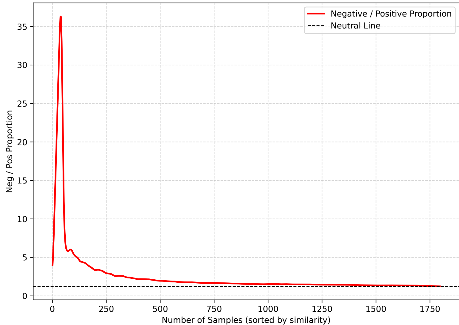
Negative/Positive Ratio along Similarity Ranking (RET)
