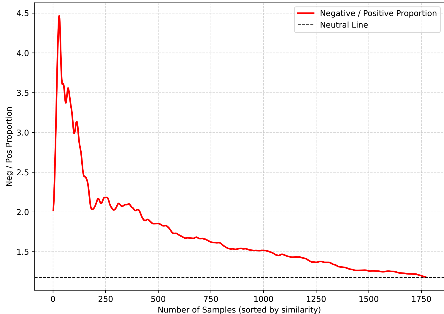
Negative/Positive Ratio along Similarity Ranking (TCF7L2)
