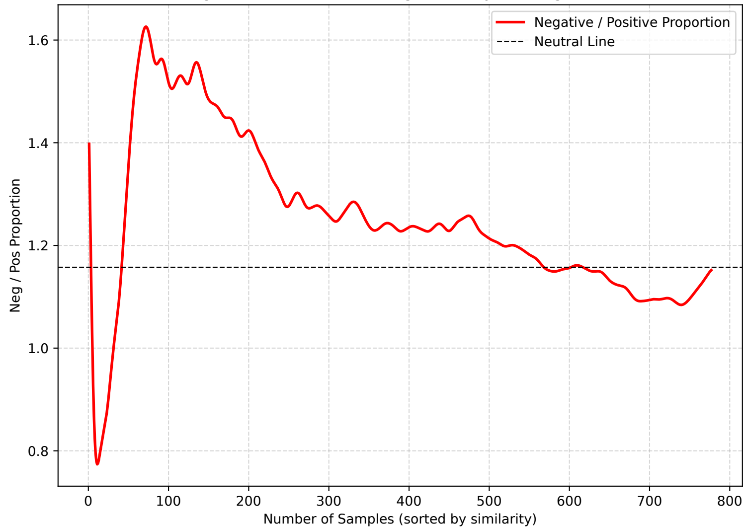
Negative/Positive Ratio along Similarity Ranking (TERT)
