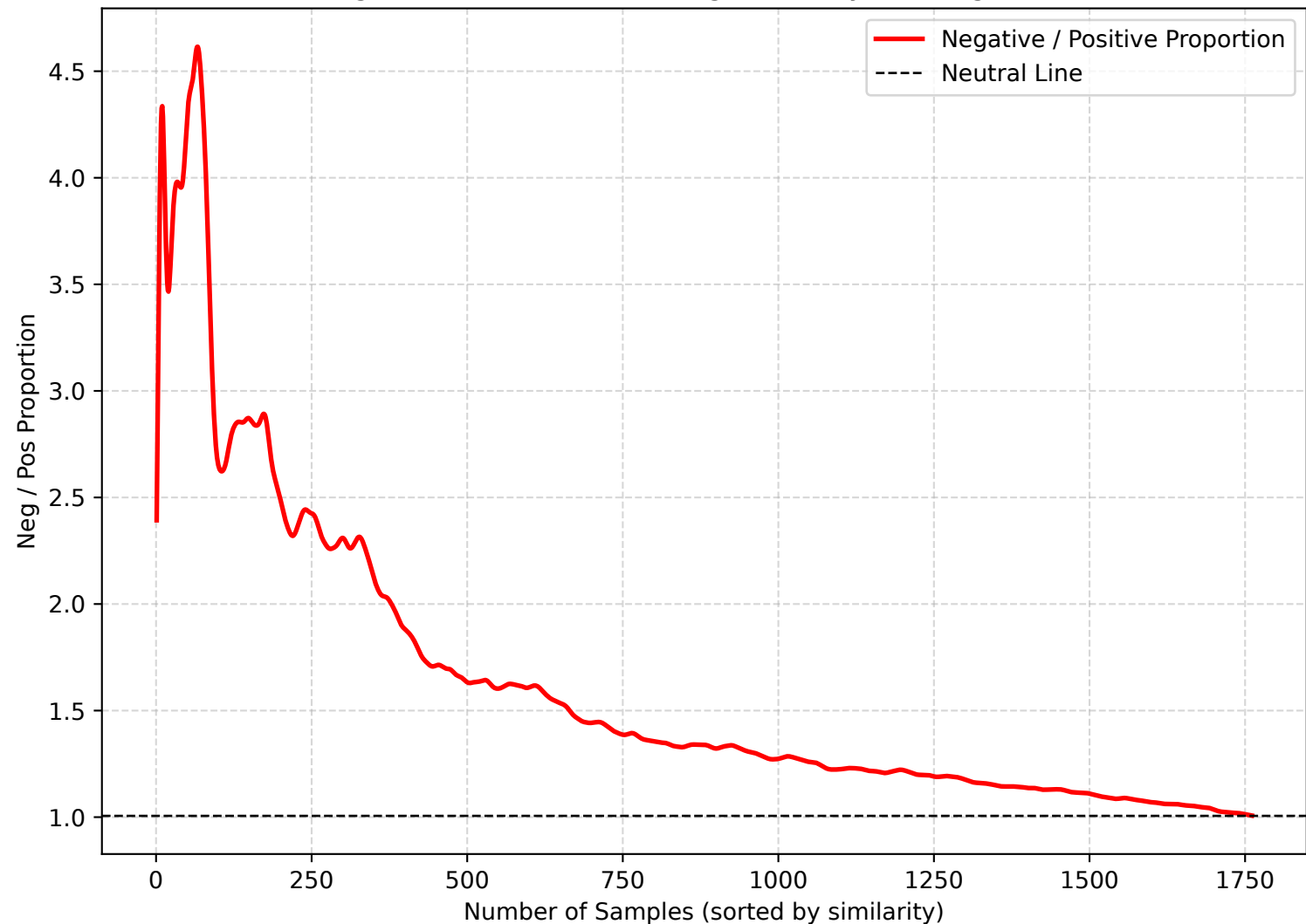
Negative/Positive Ratio along Similarity Ranking (UC88)
