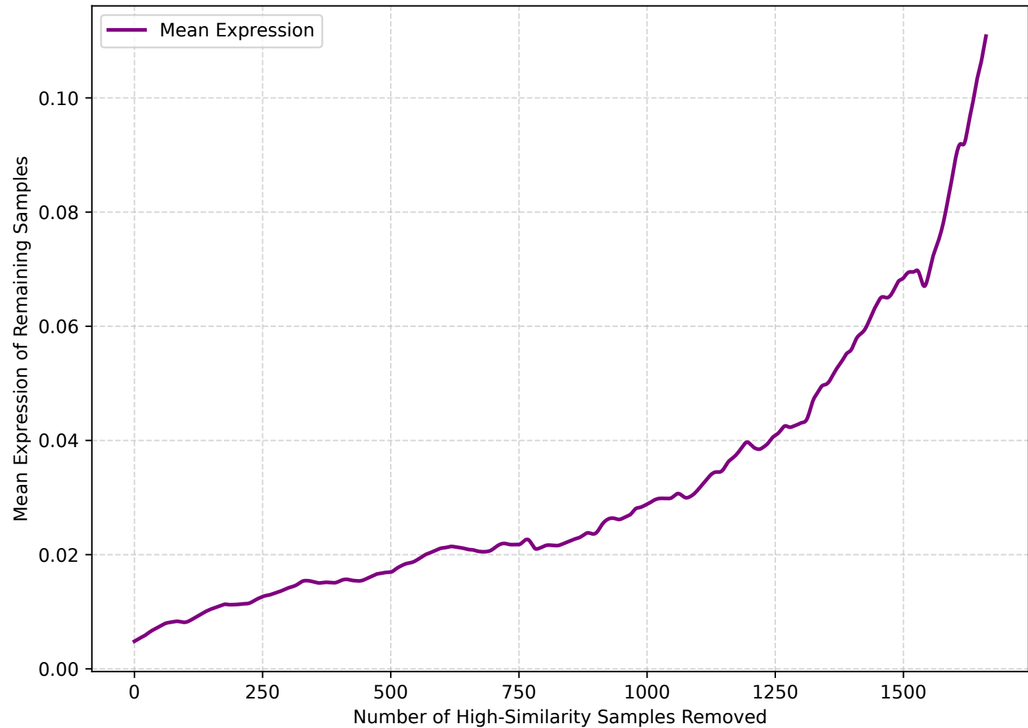
Expression Stability after Removing Top Similar Samples (UC88)
