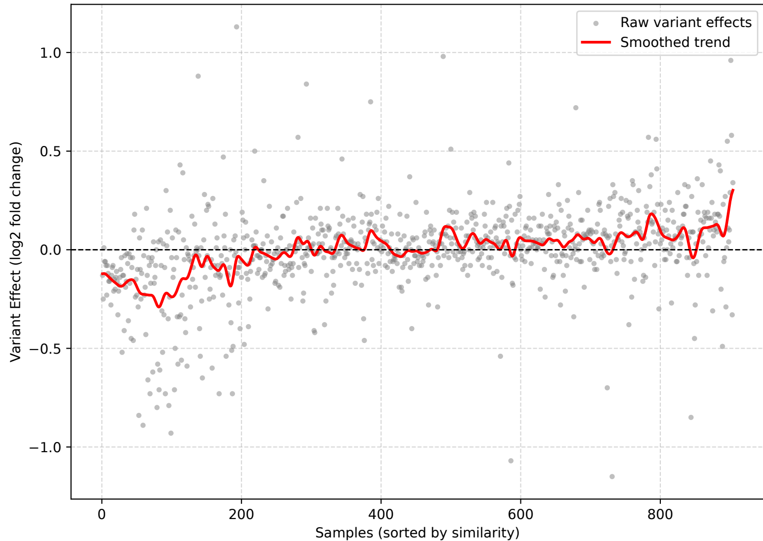
F9: Expression Trend along Similarity Rank
