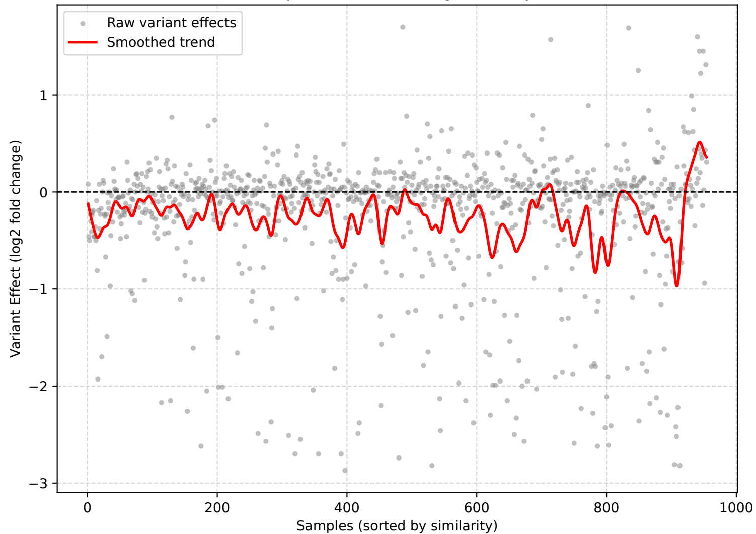
LDLR: Expression Trend along Similarity Rank
