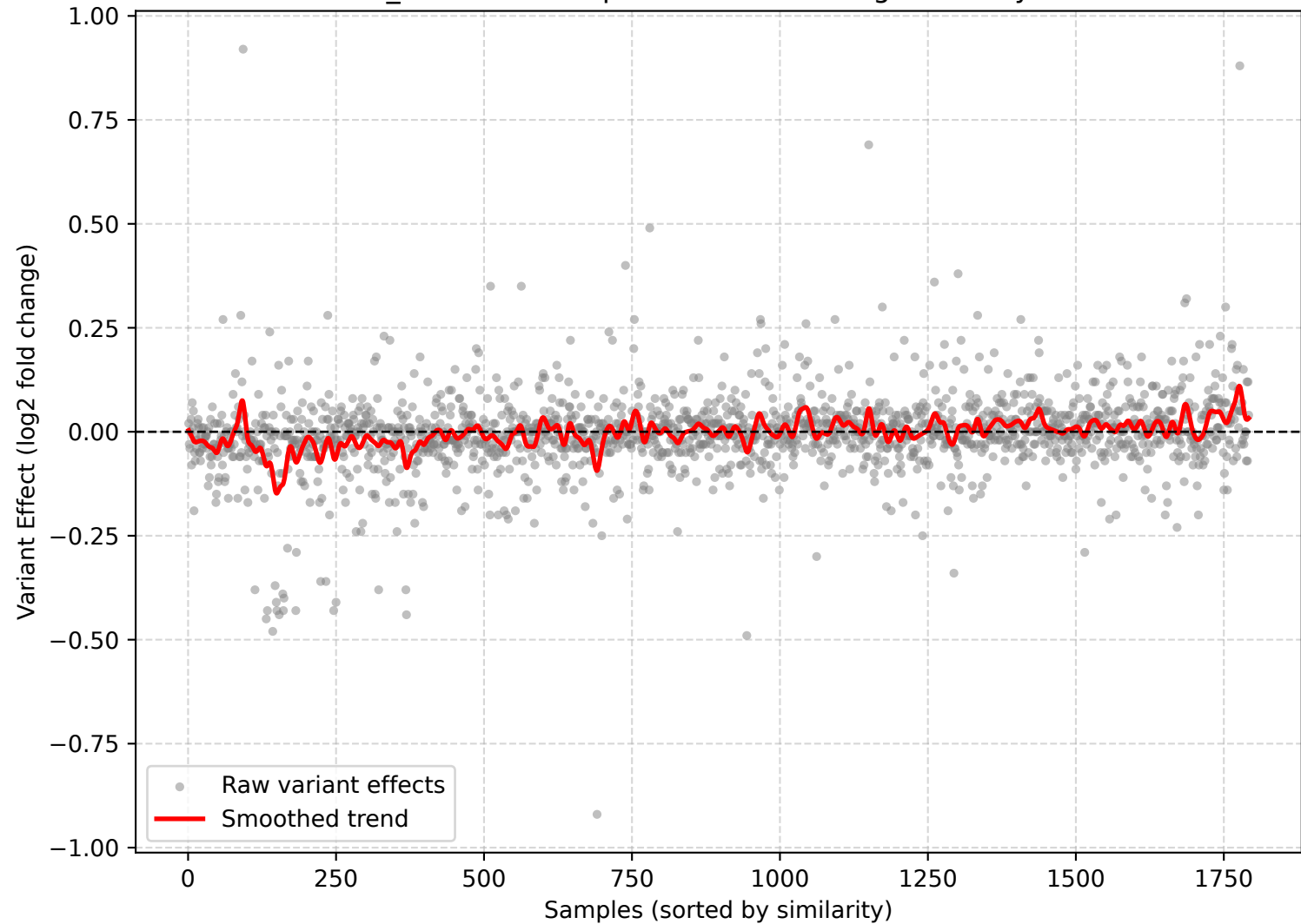
MYC_rs6983267: Expression Trend along Similarity Rank
