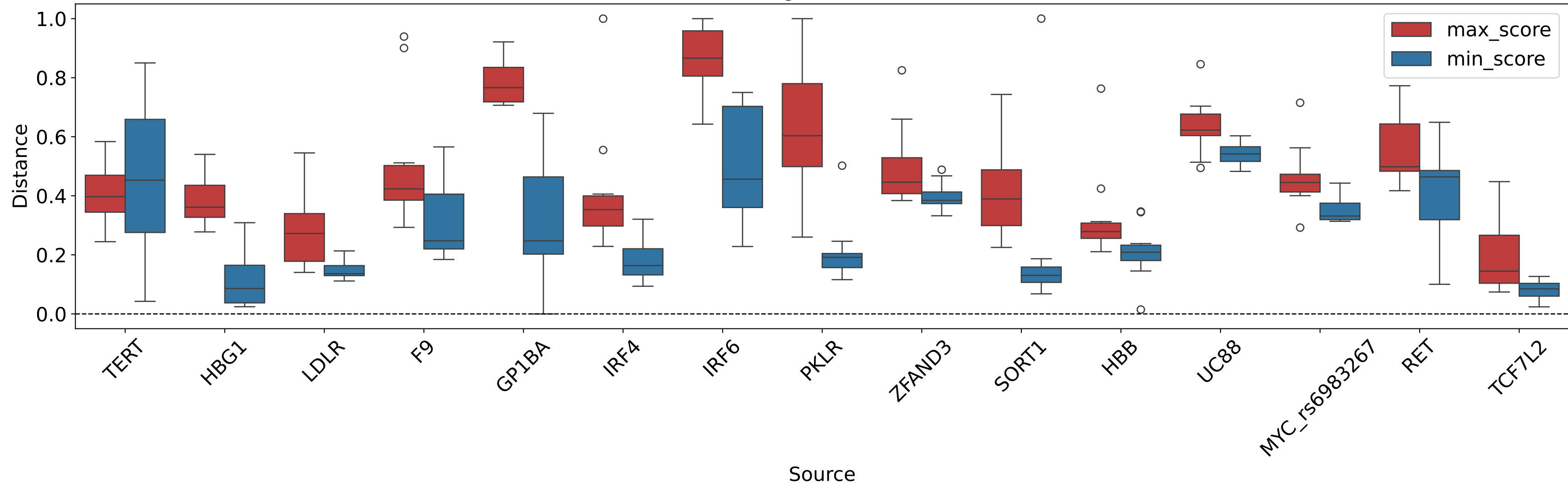
Distance: Variant vs Original (MPRABase, mahalanobis)
