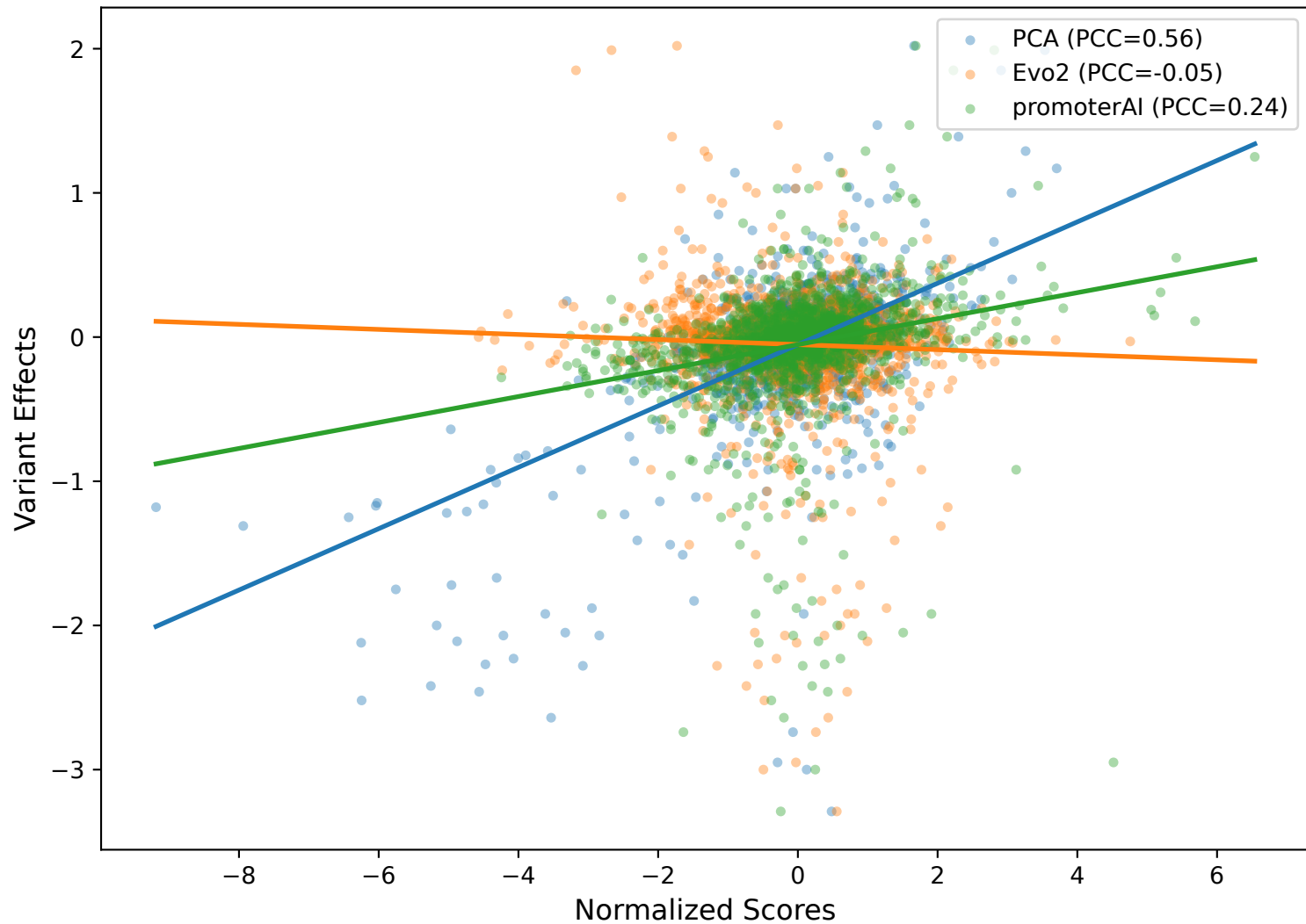
PCC Plot for IRF6
