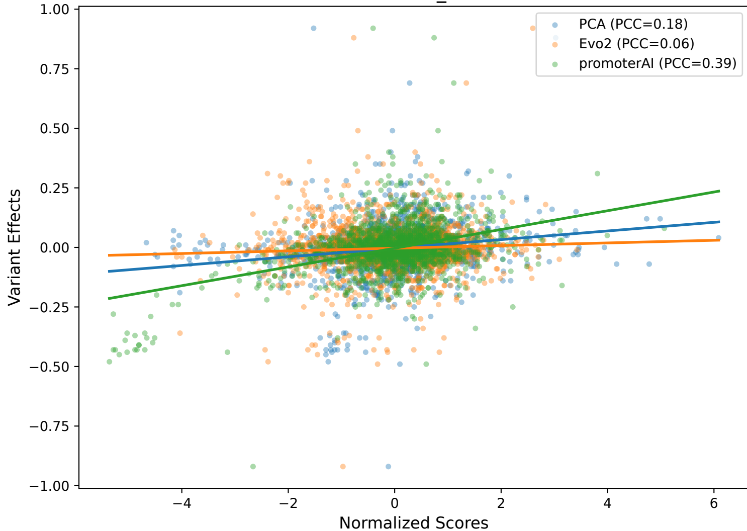
PCC Plot for MYC_rs6983267
