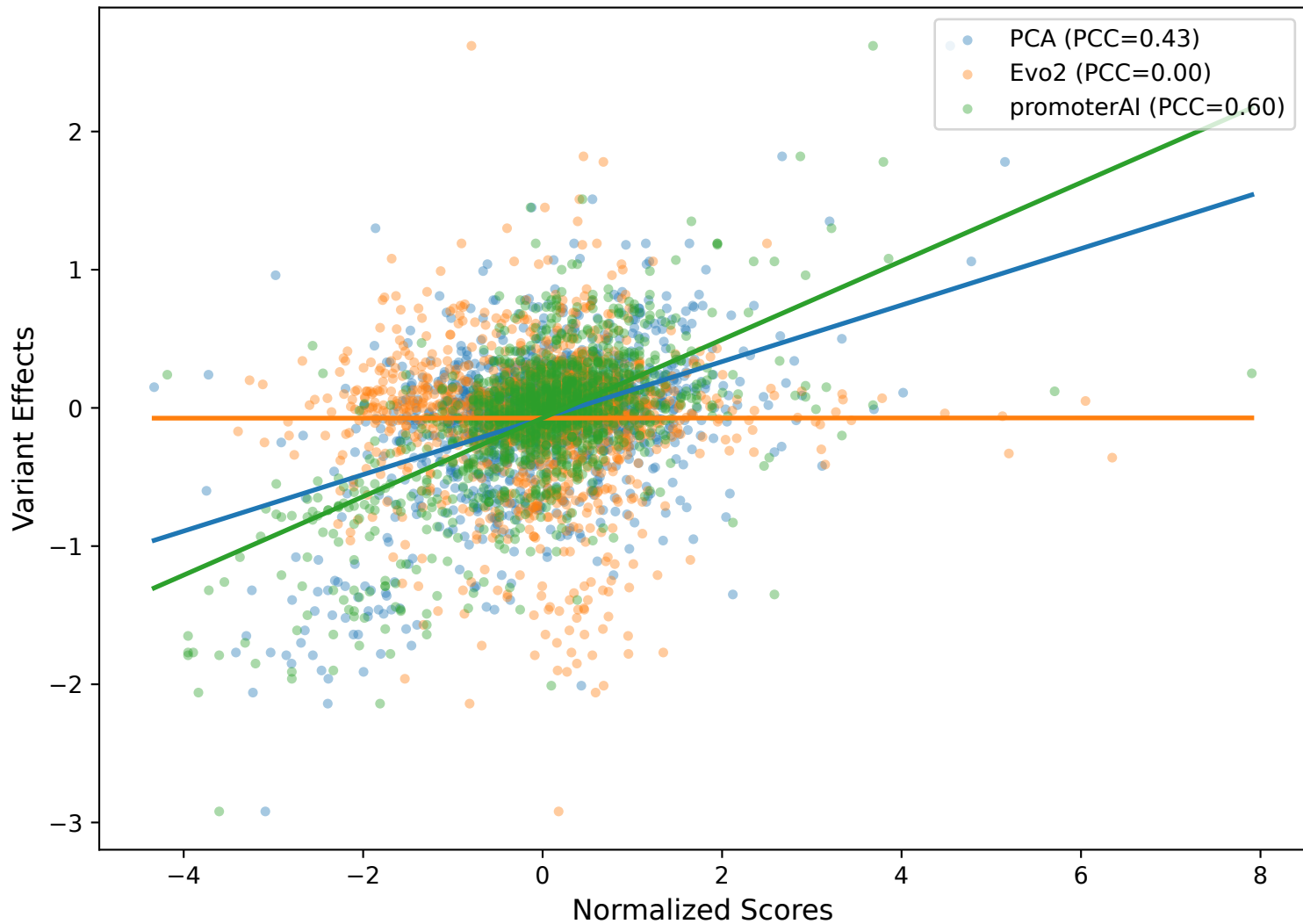
PCC Plot for PKLR
