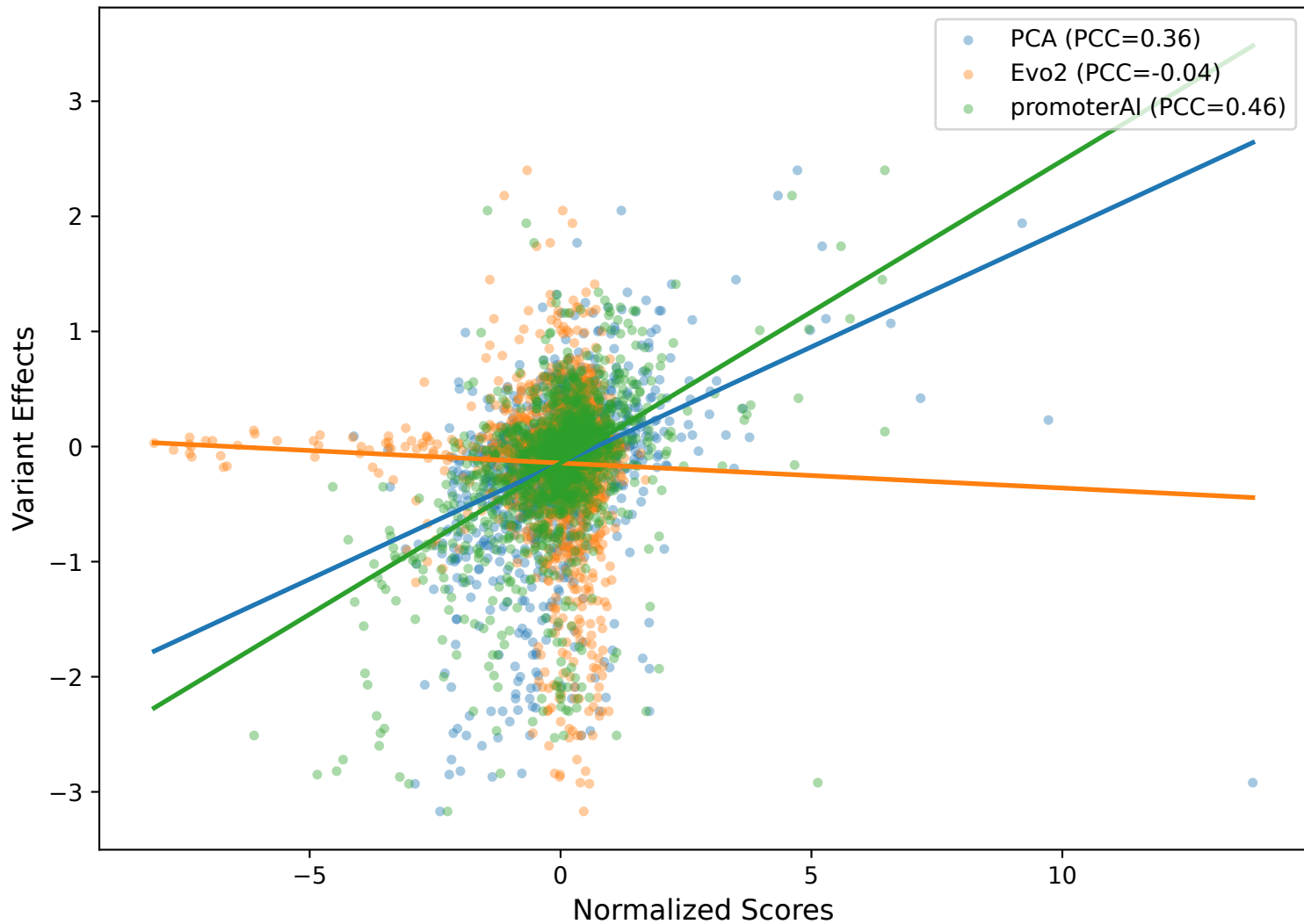
PCC Plot for SORT1
