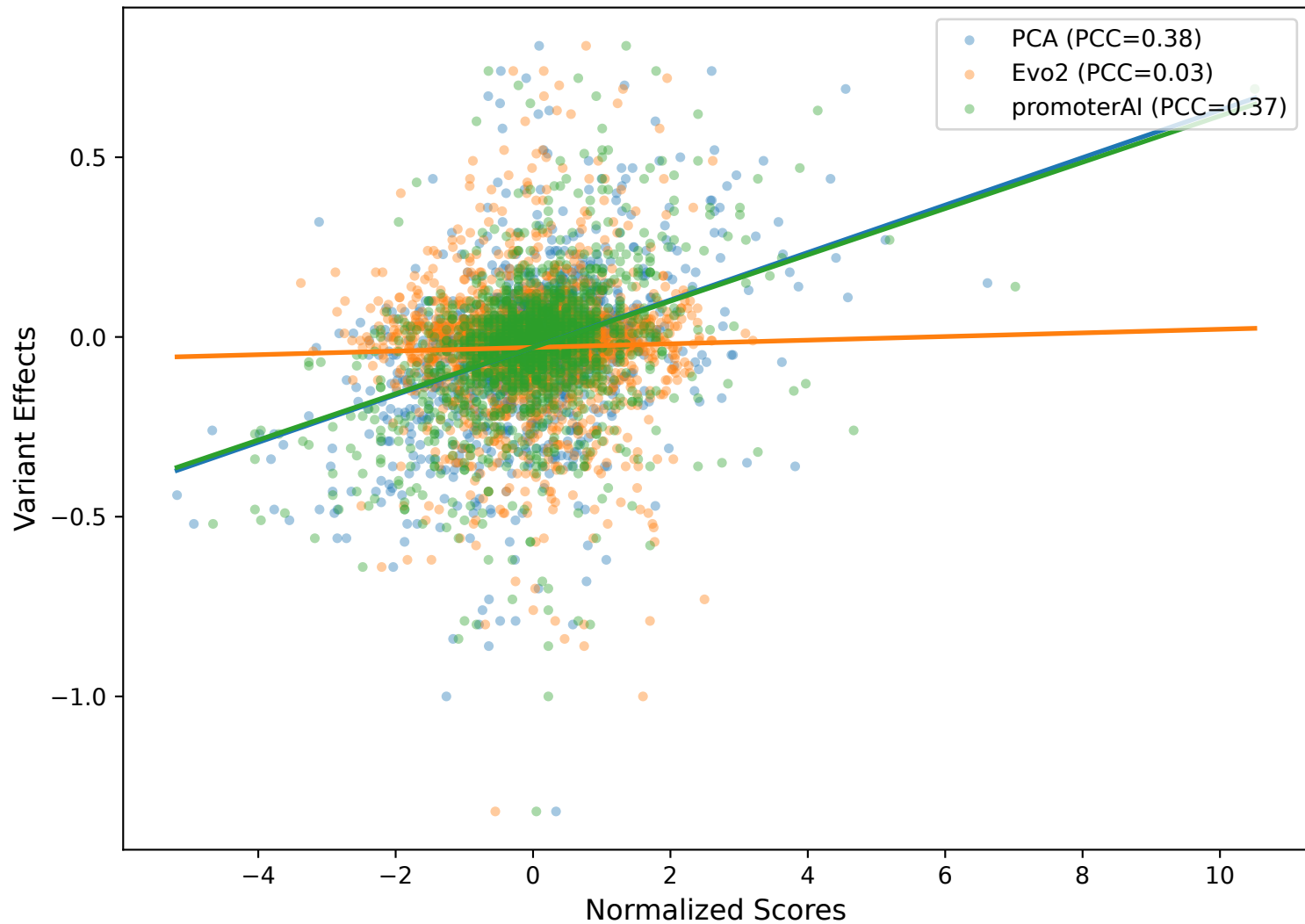
PCC Plot for ZFAND3
