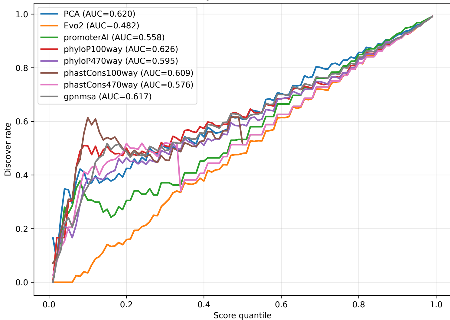
Quantile-aligned Discover Rate — HBB
