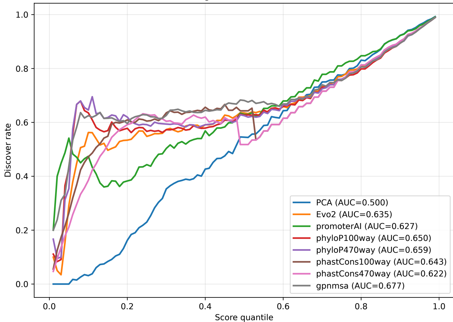
Quantile-aligned Discover Rate — LDLR
